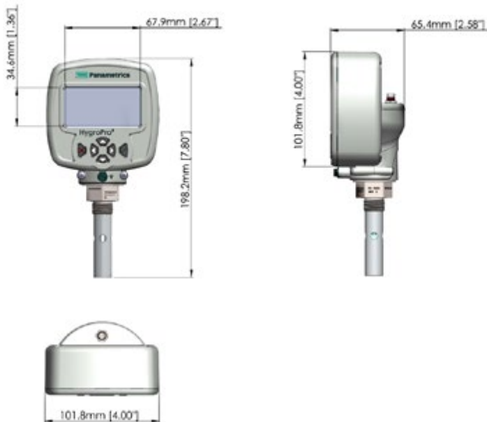
HygroPro II dimensions
