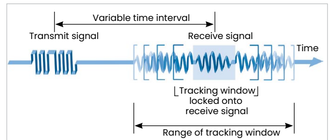
ATW ensures accuracy when fluid conditions change
