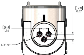
**6.24 [158.5] WEATHERPROOF VERSION
